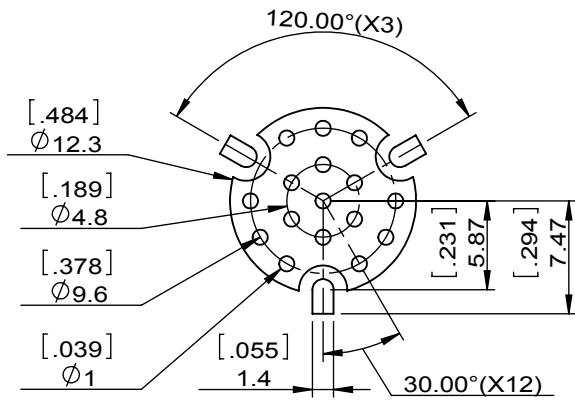
Copper Parttern
