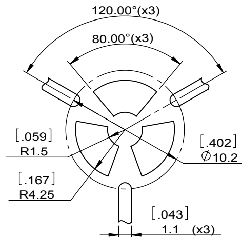
Soldermask Pattern
