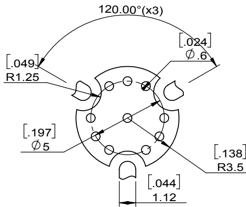
Copper Pattern
